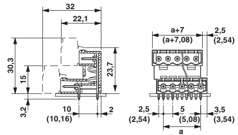
Dimensional drawing
